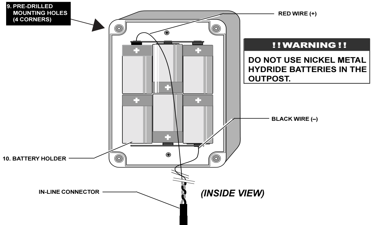
FIG-2: BOTTOM HALF OF INTERNAL HOUSING, SHOWING CELL POLARITY
